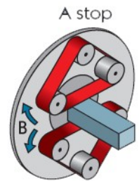
Flat parts grinding max. 20x20 mm.
