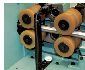
AN/A equipment for automatic abrasive belts opening with photocell
