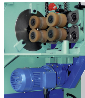
Front and rear powered self-centering feed systems with adjustable speed
